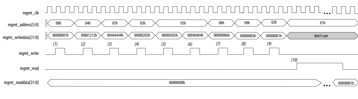
Figure 2: Waveform Example for Performing Dynamic Reconfiguration in Reconfiguring M_{FRAC} , M, N, and C Counters
